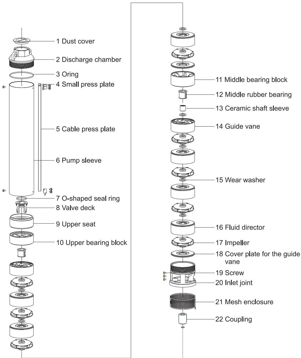
Pump Part of QJD Series
