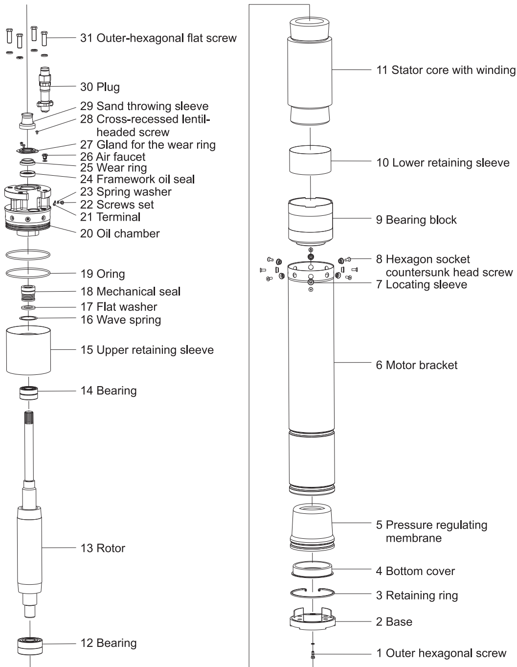
Motor Part of 6SE-T Series
