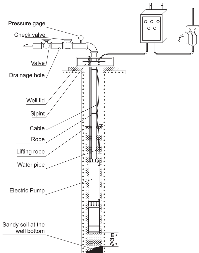
Installation Diagram
