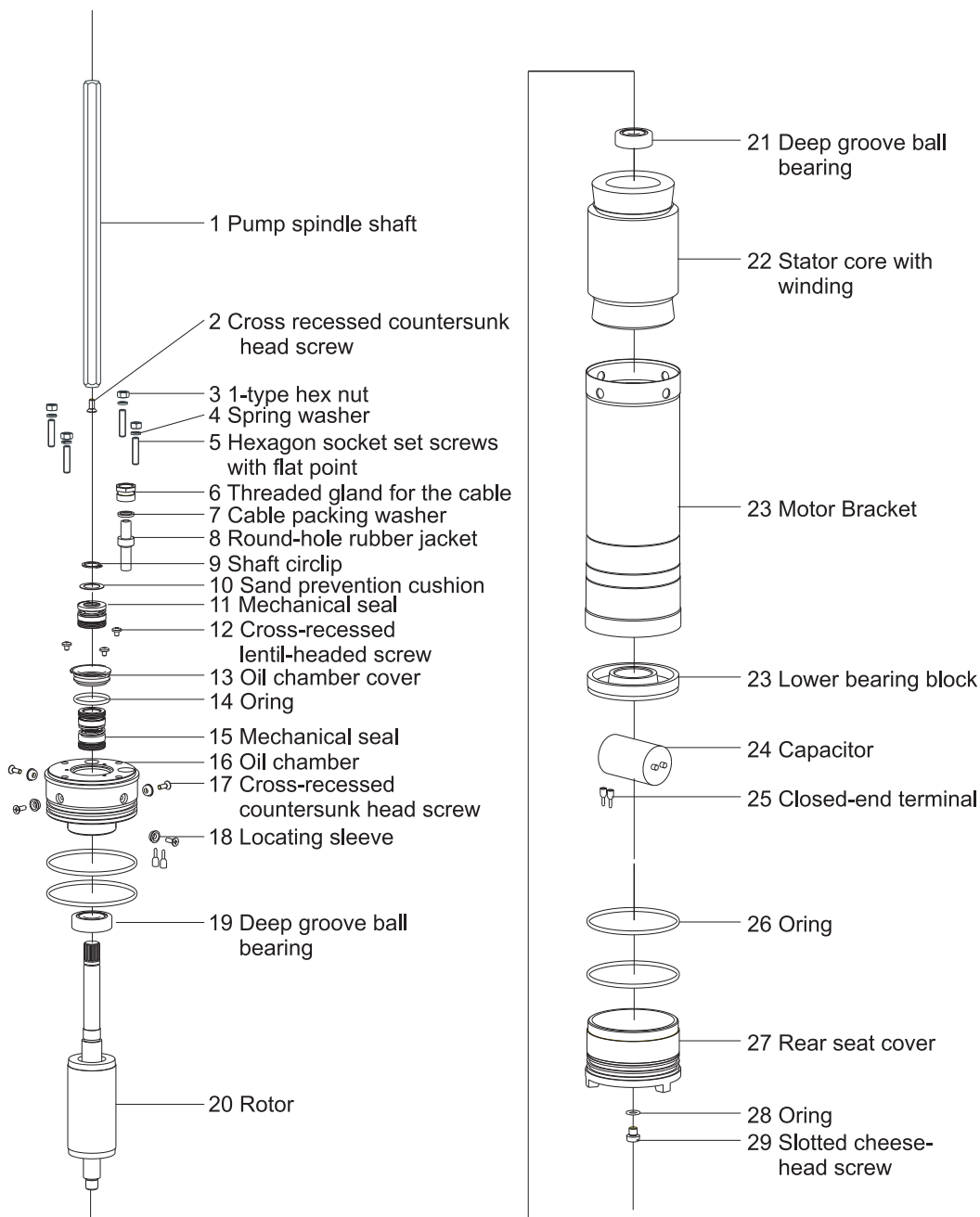
Motor Part of QJD Series
