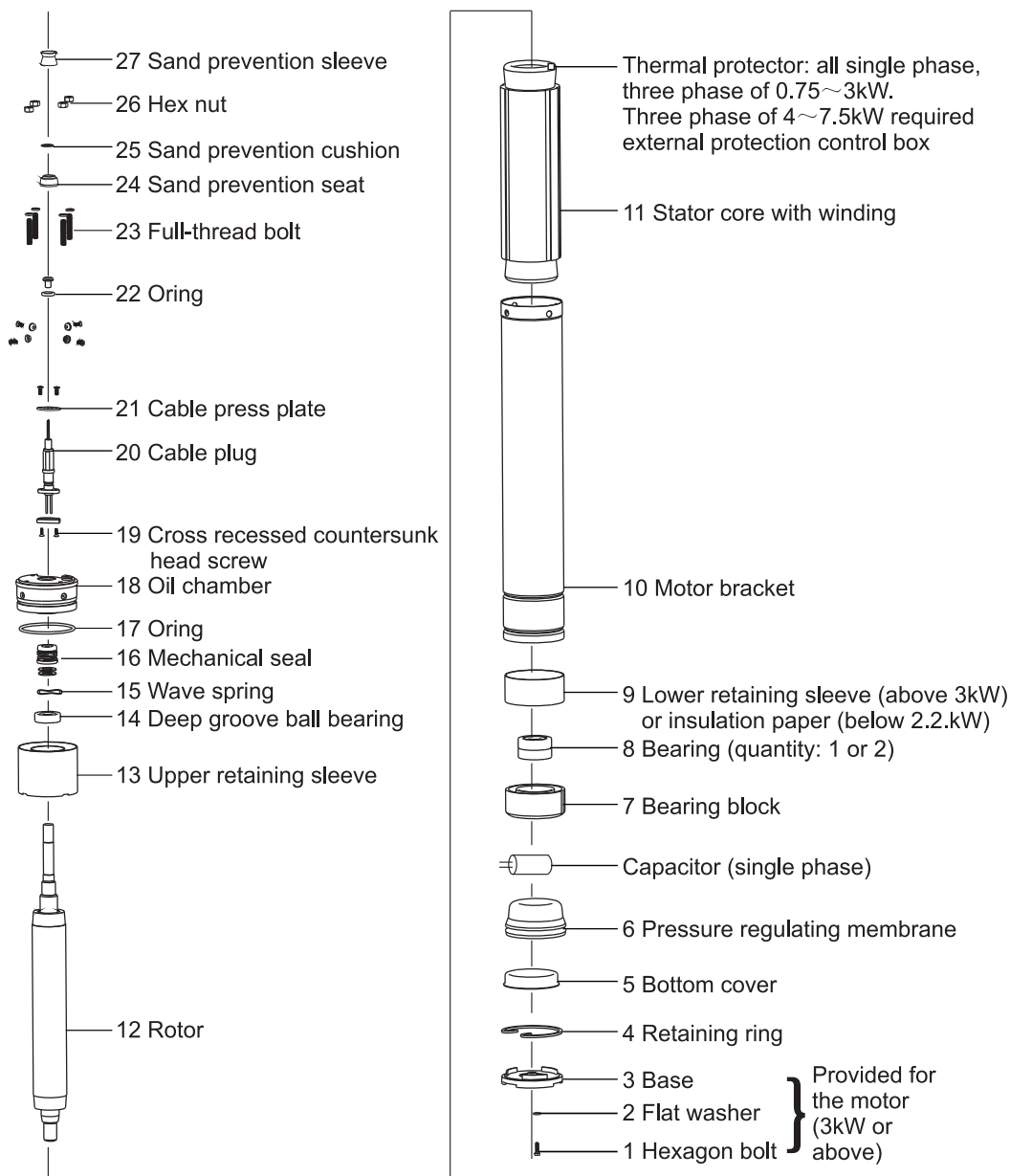
Motor Part of SE (m) Series
