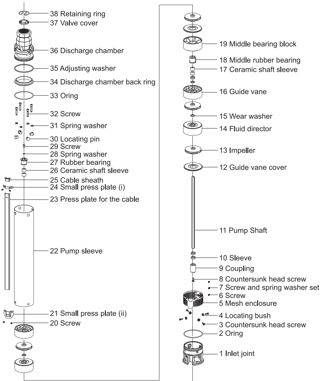
Pump Part of SE (m) Series
